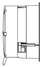
3.92" (99.6mm) Shallow Enclosure Side View
