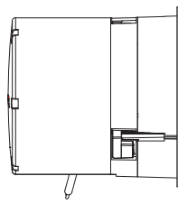
5.92" (150.4mm) Deep Enclosure Side View
