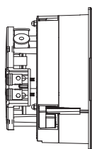
3.74" (95.1mm) Mounting Depth (Open Back) Side View
